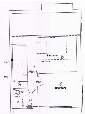
Proposed Second Floor
